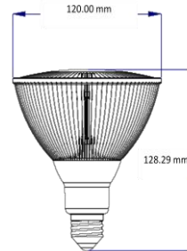
E26/24(US) Beam Angle 38°,72° ,120°,135°
