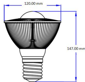
E39/41 Beam Angle 100°
