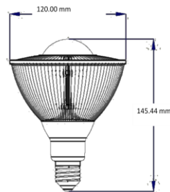
E39/41 Beam Angle 100°
